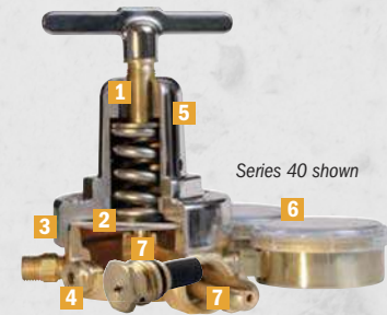
Sure Seat filtered high-pressure seat assembly
